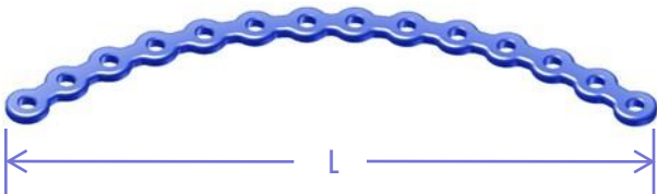
Pelvic Reconstruction Locking Plate 3.5 mm, curved
