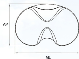
A3 GT Deep Dish Tibial Insert (UHMWPE)
