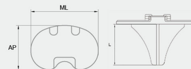
A3 Fixed Tibial Tray (Co-Cr-Mo)
