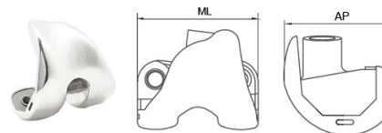
ACCK Femoral Condylar (Co-Cr-Mo)
