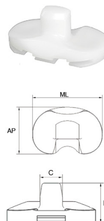
ACCK Tibial Insert (UHMWPE)
